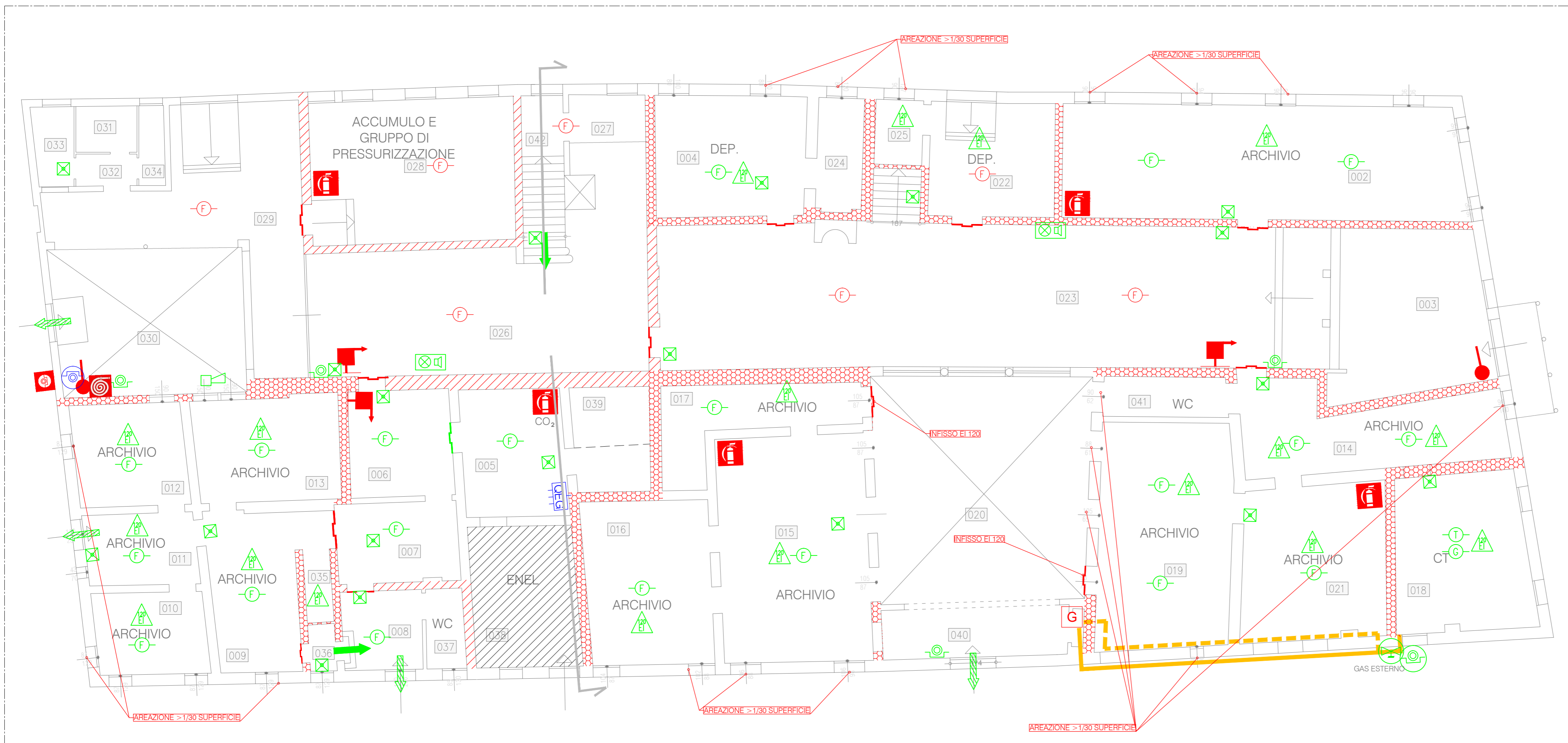
PIANO TERRA 1:100
